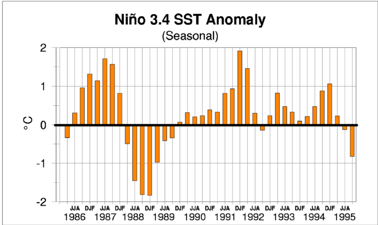
Figure 2. Seasonal eastern tropical Pacific sea surface temperature anomalies.
