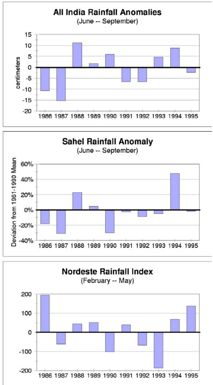
Figure 3. Regional rainfall indices
