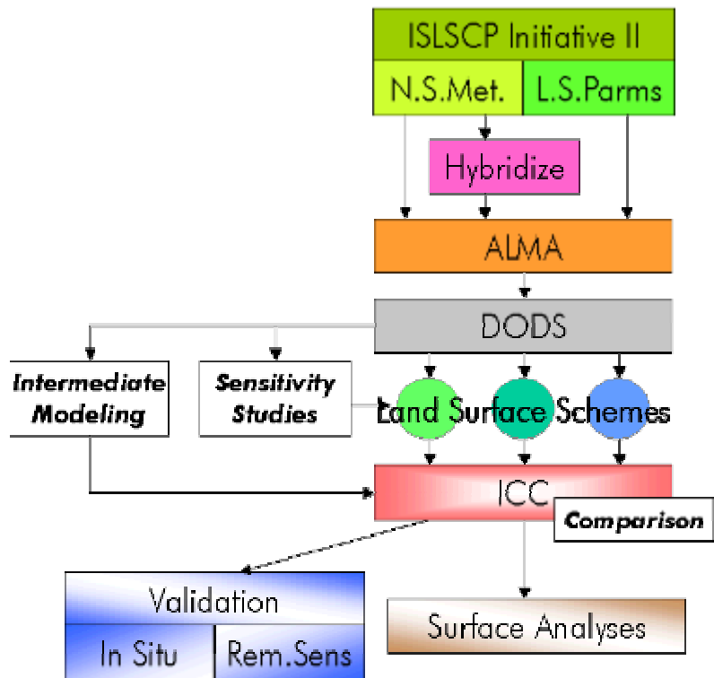
Figure 4. Implementation flowchart for GSWP-2.
