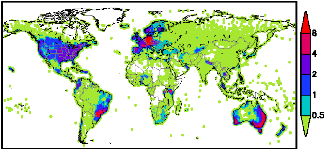
Figure 6. Example of gauge density for CRU stations for January 1986. Unshaded areas have no stations within 2° of grid box.
